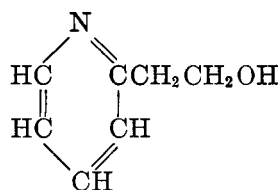
2-(1-Pyridyl)ethanol
